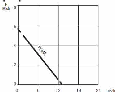
pompcurve
